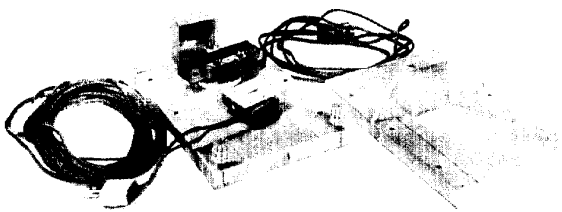
Fig. 3. Left: Photograph of the reference plate with leveling screws with autocollimation mirror, line dipole coil and peaking strip in ceramic boat. Right: Reference plate with ceramic legs and autocollimation mirror.
