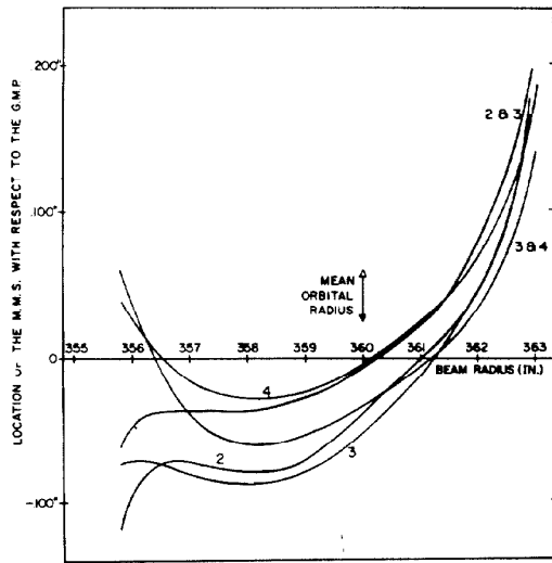
Fig. 1. This is a composite of several measurements of the magnetic median surfaces for different pairs of pole pieces. The differences in these profiles for a given pair of pole pieces were within \pm 0.020 inch. The normalizing point was reproducible within \pm 0.1 inch for any given pair.
