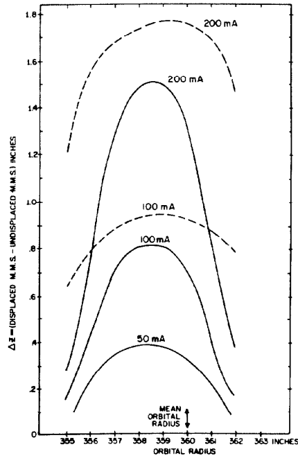
Fig. 2. Variations in the location of the magnetic median surface as a function of the intensity of current sheets on the pole pieces. Solid lines: central one third width current sheets, dashed lines: full width current sheets.
